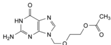
I. 2-[(2-amino-6-oxo-1,6-dihydro-9 H -purin-9-yl)methoxy]ethyl acetate,
