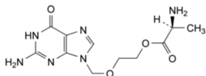
H. 2-[(2-amino-6-oxo-1,6-dihydro-9 H -purin-9-yl)methoxy]ethyl L-alaninate,
