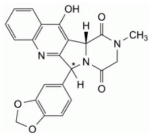
G. (12b R )-6-(1,3-benzodioxol-5-yl)-12-hydroxy-2-methyl-2,3,6,12b-tetrahydropyrazino[1',2':1,5]pyrrolo[3,4- b ]quinoline-1,4-dione,
