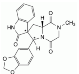
I. (8a' R )-6'-(1,3-benzodioxol-5-yl)-2'-methyl-2',3',8',8a'-tetrahydro-6' H -spiro[indole-3,7'-pyrrolo[1,2- a ]pyrazine]-1',2,4'(1 H )-trione.
